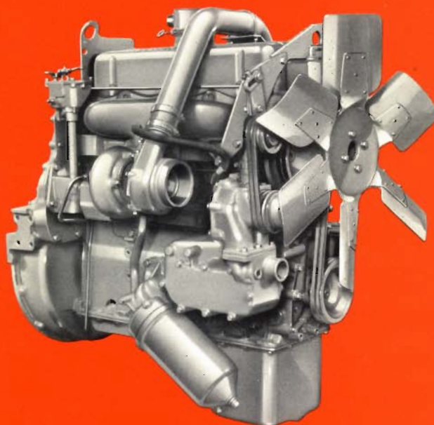
Typical 4-53T Truck Model
