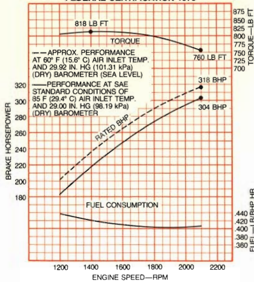
BASIC ENGINE PERFORMANCE MODEL 8V-71N WITH 7E65 INJECTORS FEDERAL CERTIFICATION 1979
